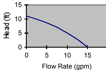
C-99 Pump Curve
